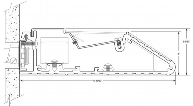
Luminaire Cross-Section
