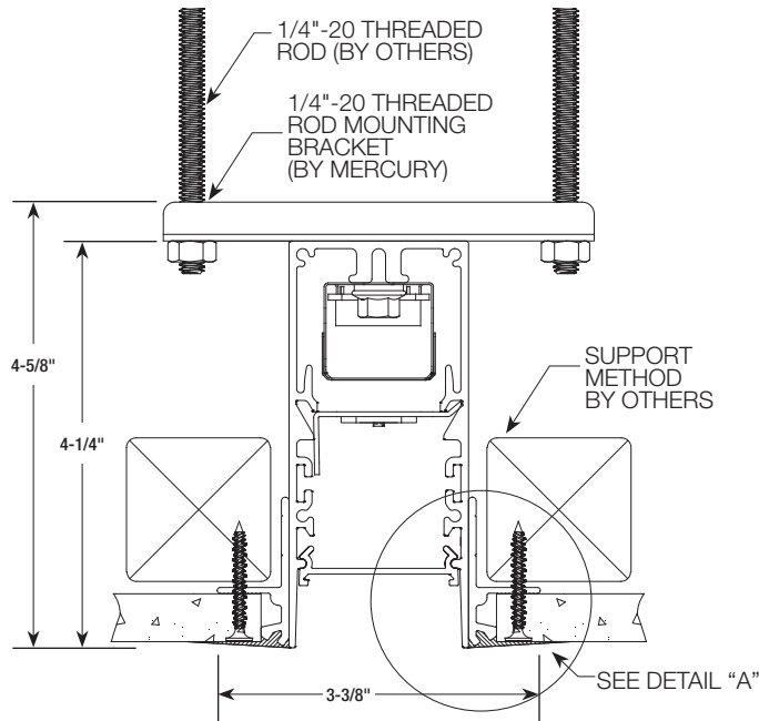
TRIMLESS FIT FOR 1/2" DRYWALL (REQUIRES PLASTERING-IN AFTER INSTALLATION BY OTHERS)
