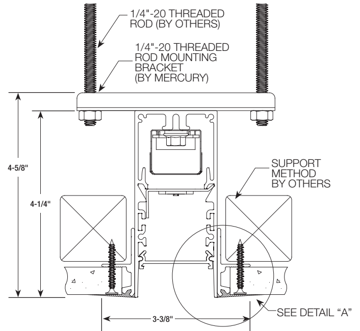
TRIMLESS FIT FOR 5/8" DRYWALL (REQUIRES PLASTERING-IN AFTER INSTALLATION BY OTHERS)
