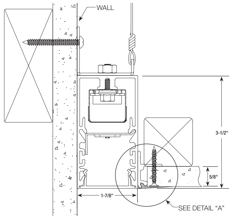
TRIMLESS FIT FOR 5/8" DRYWALL
