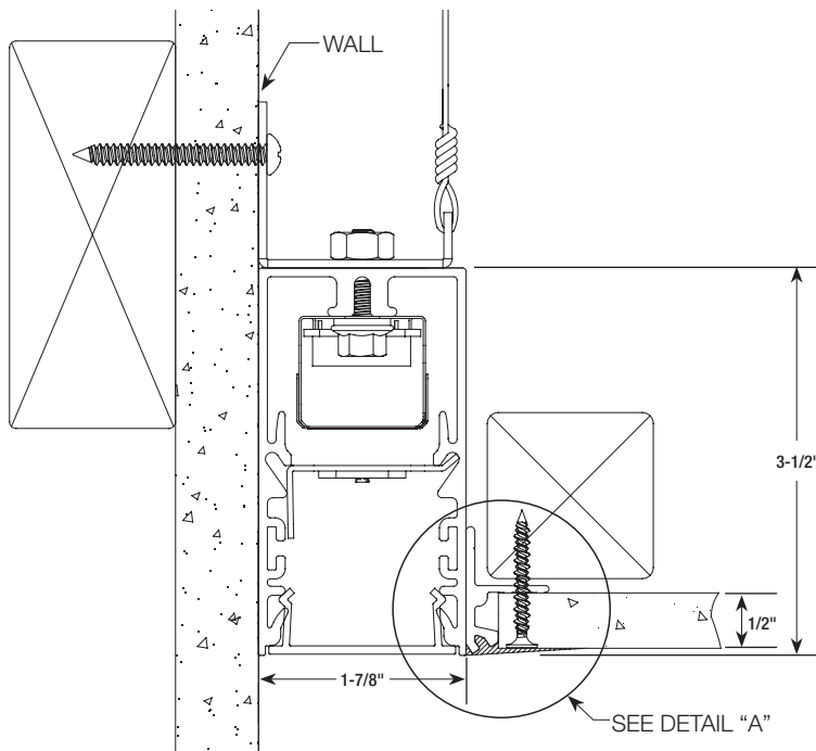
TRIMLESS FIT FOR 1/2" DRYWALL
