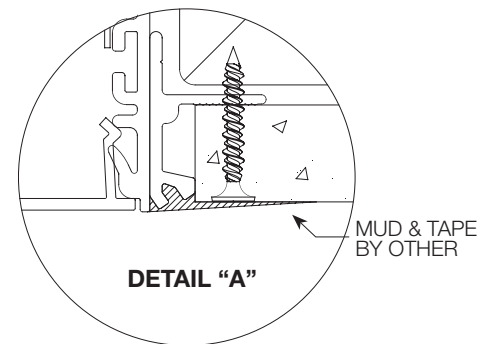
TRIMLESS FIT FOR 5/8" DRYWALL
