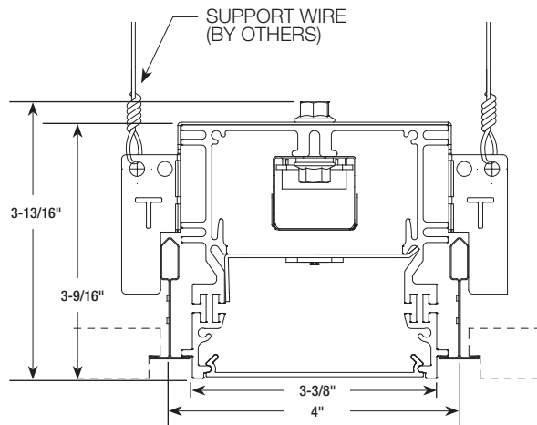
S 9/16" GRID TEGULAR TILE
